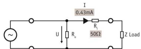
Fig. 2: Current correct measurement Preferred, when voltage drop over R_i is very small compared to the voltage drop over Z. Power loss in R_i : 9.2 μW
