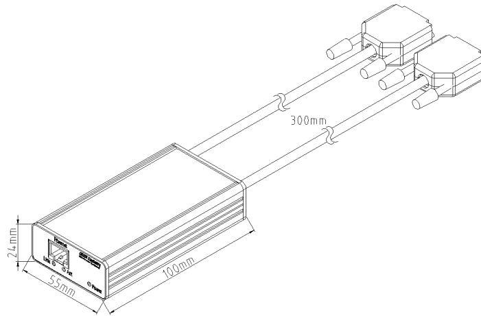
Figure 40: L95-Z318, L45-Z318, L50-Z318 - supply via LMG
