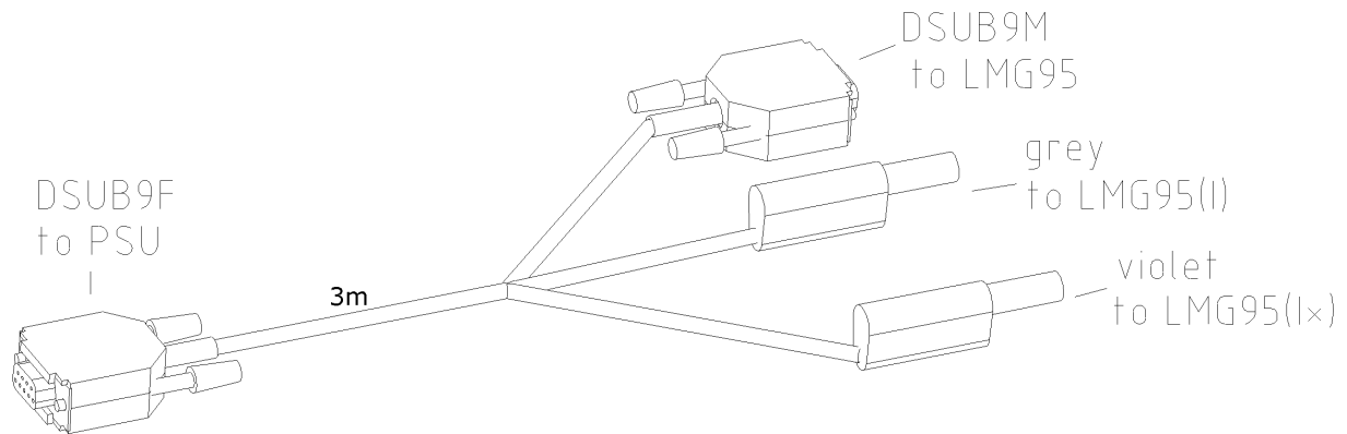
Figure 26: PSU/PCT-K-L95, for direct connection of the PSU60/200/400/700 and PCT200/600 to the current input of the LMG95
