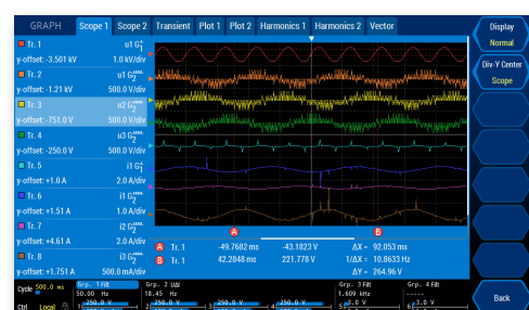
Display of sampling values of 8 signals in two scopes
